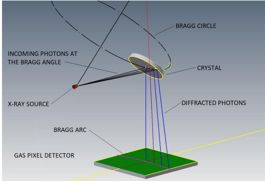
Fig 4 Geometry of Bragg diffraction for monochromatic photons.
