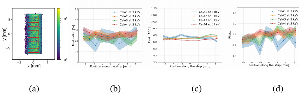
Fig 13 Comparison of strip analysis of four CalA models for Ag fluorescence emission at 3 keV in TV. The shaded area represents the error in the measurement. (a) Subdivisions of the strip for analysis highlighted in red; (b) modulation as a function of position along the strip; (c) energy peak in ADC as a function of position along the strip; (d) phase as a function of position along the strip.
