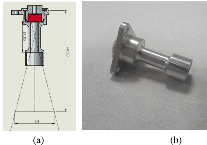
Fig 6 CalC illuminates the entire GPD surface with monochromatic unpolarized photons. (a) Cross-sectional view of CalC: the 55 Fe radioactive source is shown in red. Numbers are in mm. (b) Picture of CalC.
